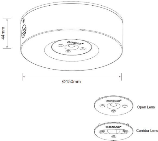
Dimension Diagram
